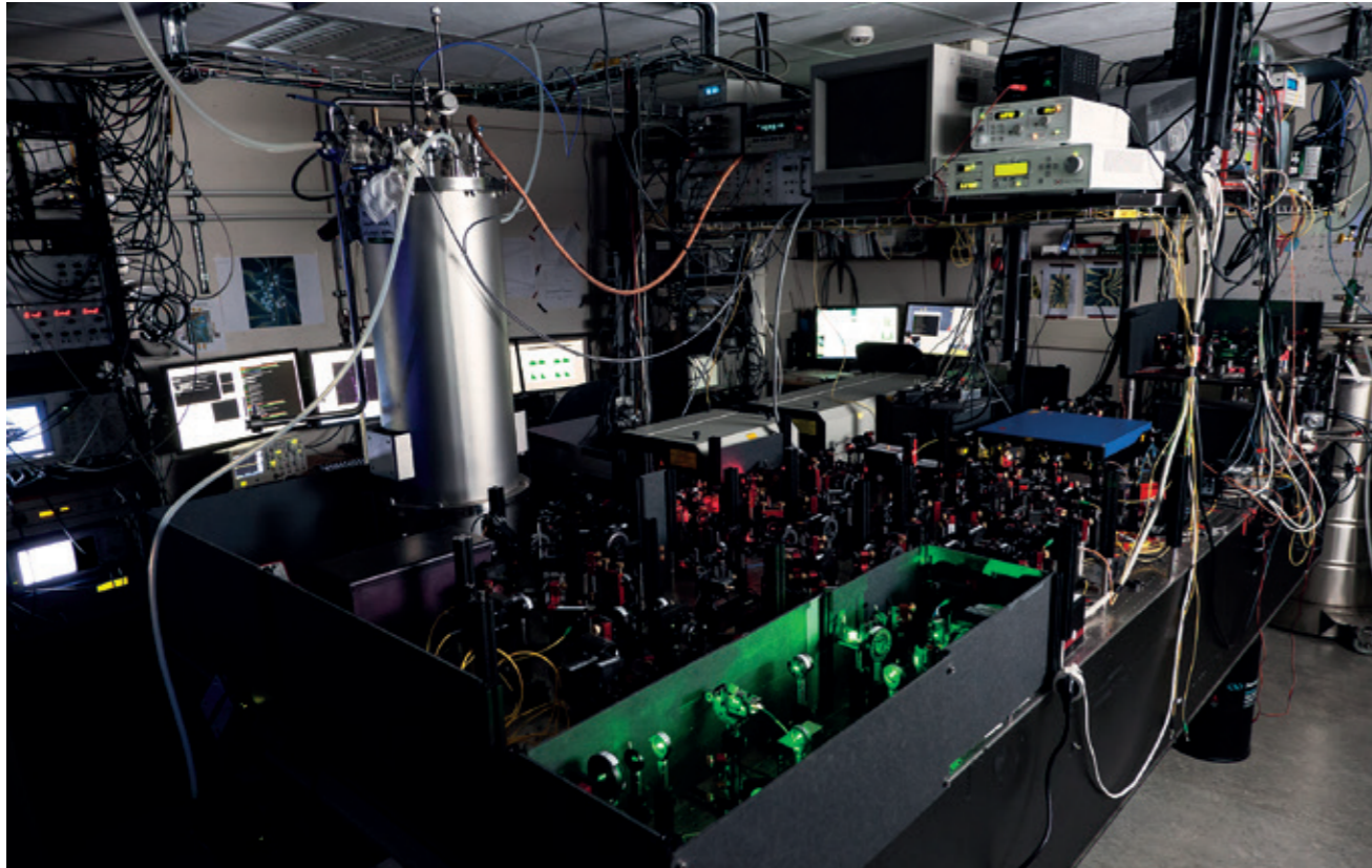
One of the endpoints or quantum nodes of the quantum link between Delft and The Hague, which is to be extended to cover the western conurbation and in due course possibly the whole of the Netherlands, en route to an entanglement-based quantum internet infrastructure. (Source: QuTech)
