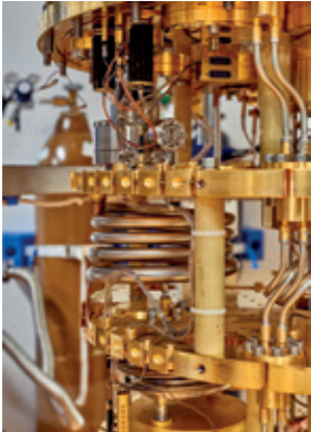
FOTO COVER A highly sophisticated 'cryostat' cooling system, in which qubits are cooled to -273°C. Extremely low temperatures are required for qubits to retain a quantum state for long enough to enable them to be used for calculations.
